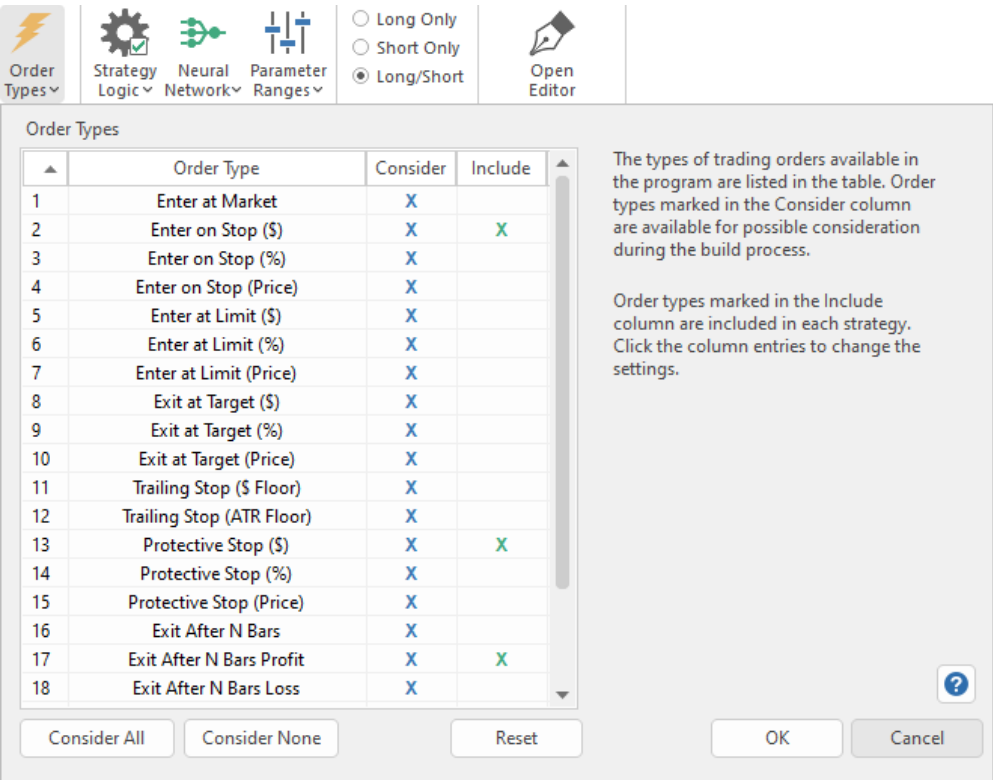
Figure 2.8. The types of trading orders available in Builder are listed on the Order Types window. Order types can be added or removed from the build set using the Consider column and added to each strategy using the Include column.
