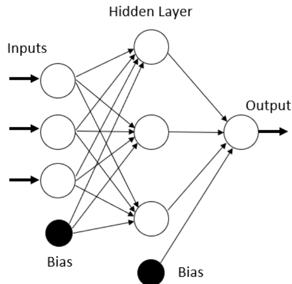
Figure 1.4. A neural network with a single output and one hidden layer. It includes three input nodes, three nodes in the hidden layer, and two bias nodes.
