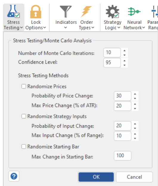
Figure 5.5. Stress testing/Monte Carlo analysis options.
