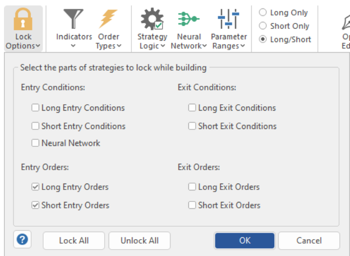
Figure 5.6. Strategy lock options.
