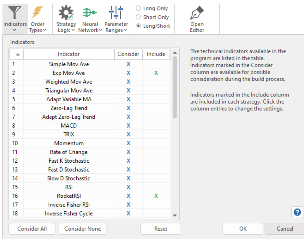
Figure 2.7. The indicators available in Builder are listed on the Indicators window. Indicators can be removed from the build set by un-checking the item in the Consider column and added to each strategy using the Include column.
