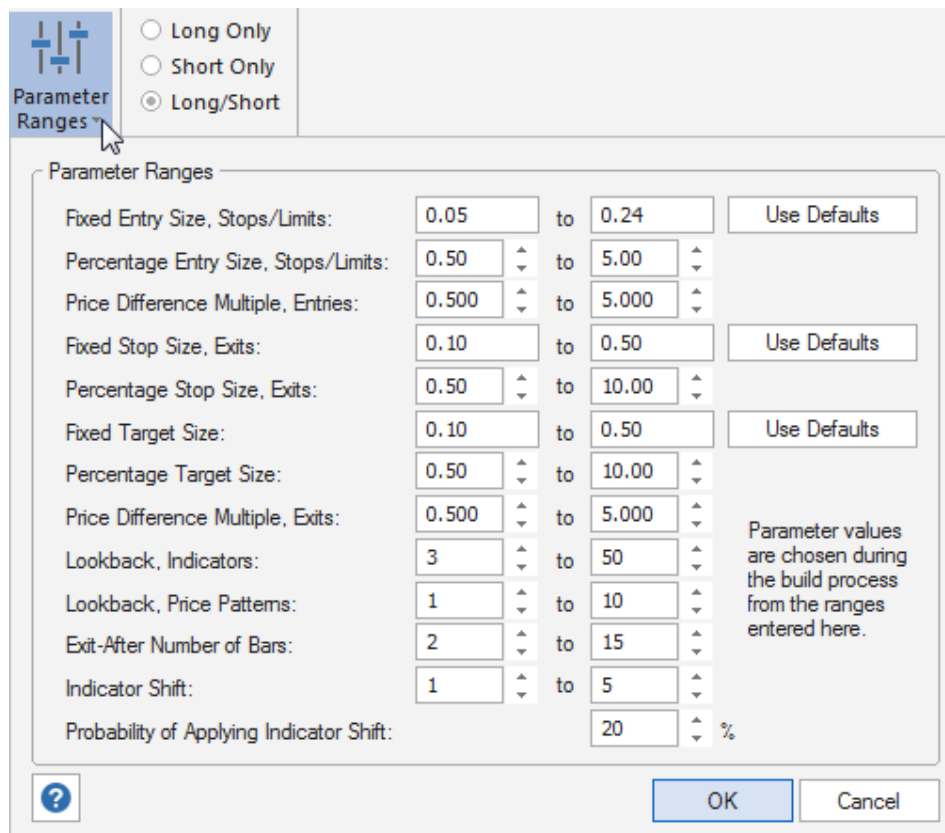
Figure 5.8. The Parameter Ranges drop-down window of the Build menu.
