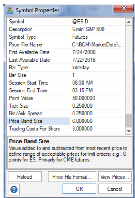
Figure 2.3. Symbol Properties window.
