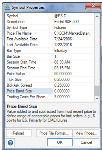
Figure 3.3. Symbol Properties window.
