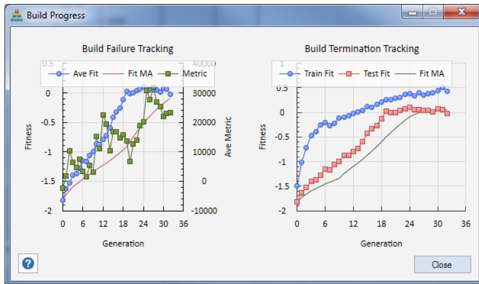
Figure 6.1. The Build Progress window displays and updates the Build Failure Tracking and Build Termination Tracking plots while strategies are being built.
