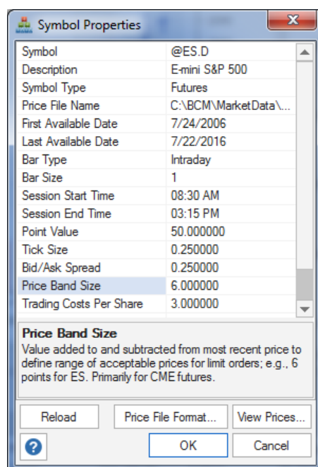
Figure 3.3. Symbol Properties window.
