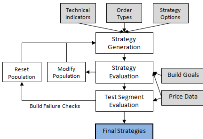
Figure 1.2. Build algorithm in Adaptrade Builder.
